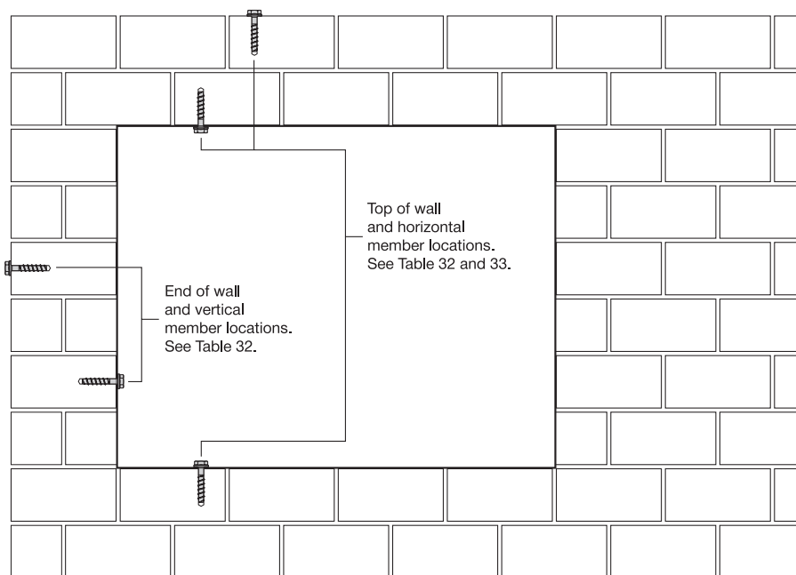
Figure 7 – Anchor locations in end of wall or wall opening applications
