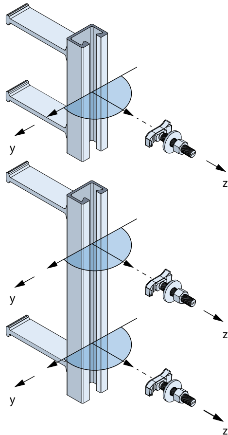
Illustration of loading directions
