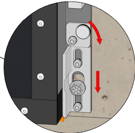
GASKET PROTECTION FEATURE
