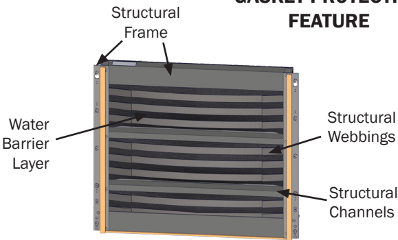
BACK VIEW (4FT FCD)
