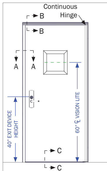
Wet-Side Elevation (RHR Swing Shown)
